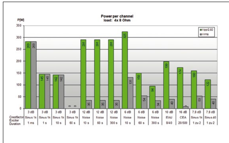
FIG. 14: The Blaze 504's power at 8 Ω per channel with simultaneous load of all channels; results for different signal types (power scale 0–350 W)
