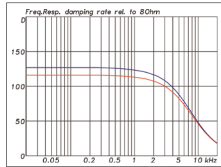
FIG. 02: Damping factor measured exemplarily for two channels, related to an 8-Ω load. The slightly different values might be caused by small contact resistances at the loudspeaker terminals
