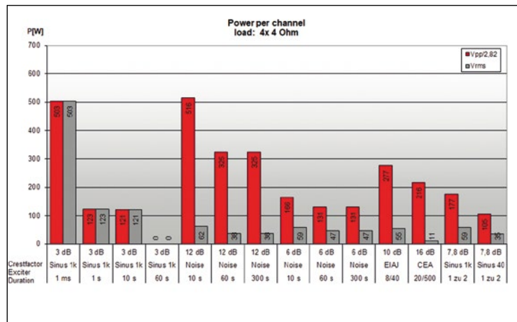
FIG. 15: The Blaze 504's power at 4 Ω per channel with simultaneous load of all channels; results for different signal types (power scale 0–700 W)
