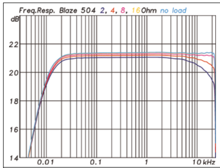
FIG. 01: Frequency responses measured with loads of 2, 4, 8 and 16 Ω and at no load
