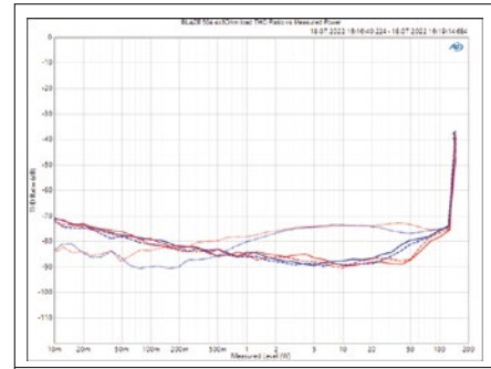
FIG. 06: Total harmonic distortion (THD) as a function of output power (x-axis in W) at a load of 4 \times 8 \Omega . Measurements at 100 Hz (- - -), 1 kHz (—) and 6,3 kHz (· · ·)
