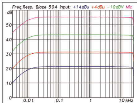
FIG. 03: Frequency response and gain depending on the selected input sensitivity. Possible settings are +14 dBu, +4 dBu, -10 dBV and mic (from bottom to top). The gain then is 21.1 dB, 31.3 dB, 43.1 dB or 55.4 dB
